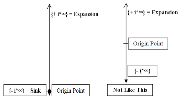
Fig. 1. Upward Absolute Infinite Imaginary Line and its Dark Shadow (Downward Absolute Infinitesimal Point)
