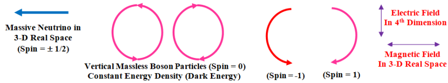
Fig. 17. Nature of Neutrinos and Vertical Massless Bosons Particles
