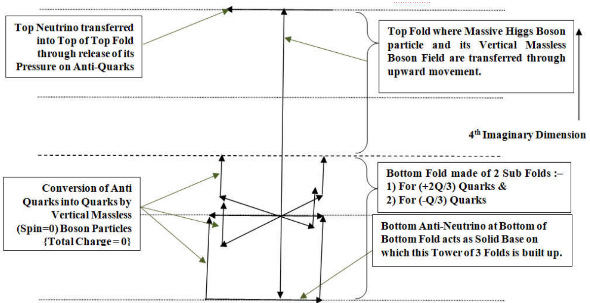
Fig. 11. Creation of Top Fold above Bottom Fold and Conversion of L.H. Anti Quarks into Quarks
