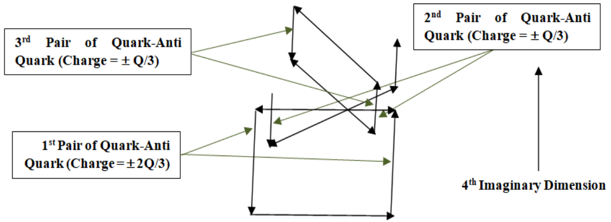
Fig. 10. Creation of 3 rd Dimension and 3 Pairs of Quark-Anti Quark
