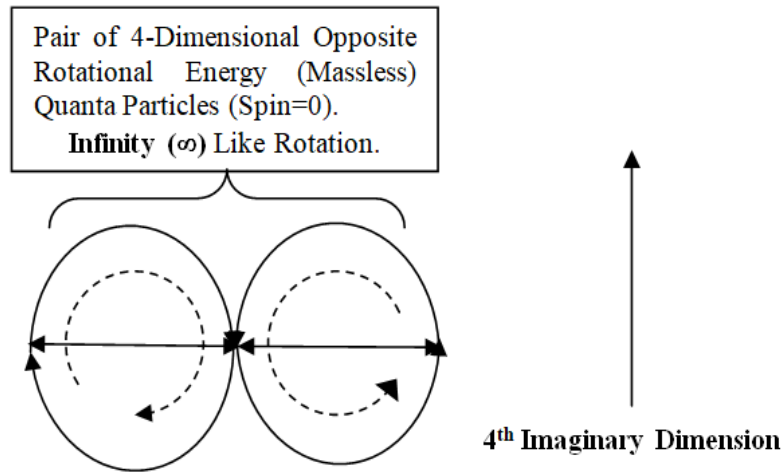
Fig. 6. Rotational Symmetry was achieved through Infinity (∞) Like Rotation (Spin=0)
