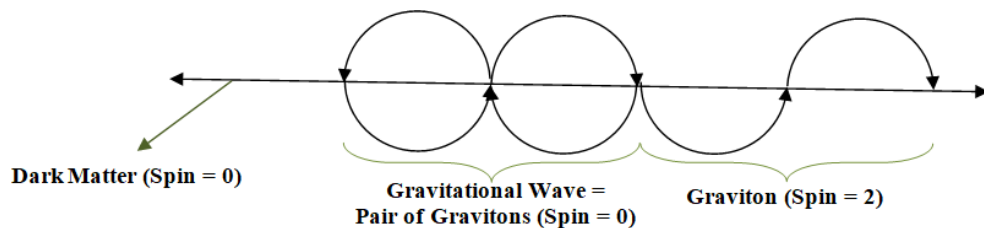
Fig. 13. Gravitational Waves (Spin= 0) made of Pair of Gravitons (Spin= ±2)
