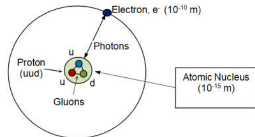
Fig. 4. Hydrogen Atom
