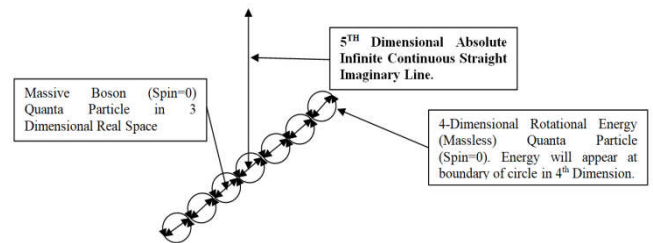
Fig. 2. Creation of 4-Dimensional Universe through Separation from 5 th Dimensional Absolute Infinite Continuous Straight Imaginary Line
