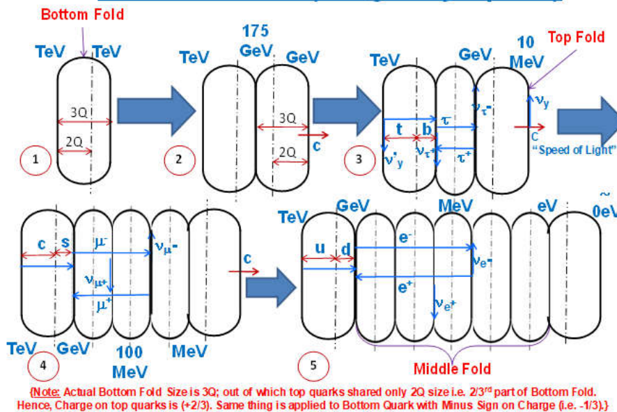
Fig. 15. Creation of Universe (3 Folds Way) in 4th Dimensional Imaginary Space
