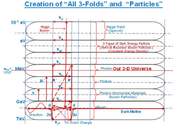
Fig. 18. Gluon, Photon, Ordinary Matter (Fermions), Graviton, Dark Matter, and 3 Types of Dark Energy
