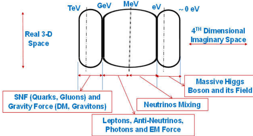
Fig. 14. Position of Particles (3 Folded Way) in 4th Dimensional Imaginary Space
