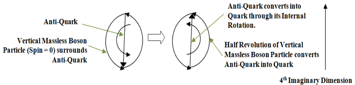
Fig. 12. Conversion of Anti-Quarks (Anti-Matter) into Quarks (Matter)
