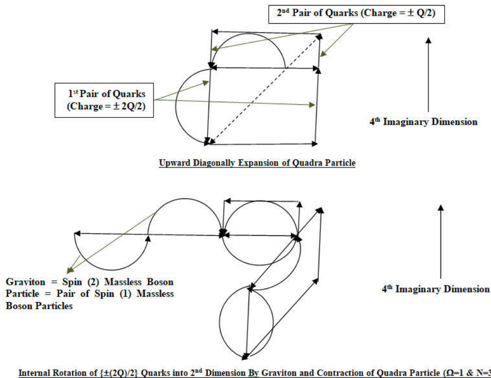
Fig. 9. Creation of 2 nd Dimension and 2 Pairs of Quark-Anti Quark
