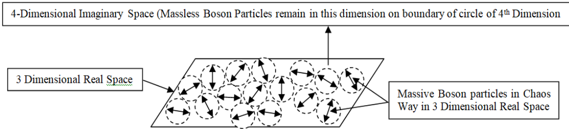
Fig. 5. Chaos of Massive Boson Particles in 3-Dimensional Real Space (Seeds of the Materialistic Visible Universe)
